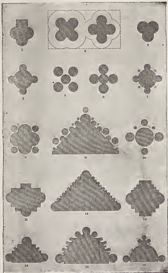
PLATE II: PLANS OF PIERS
